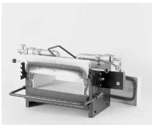
Art. ID15592 External measures: L 410 mm - H 255 mm - P 255 mm Internal measures: L 300 mm - H 250 mm - P 90 mm
