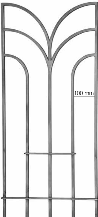
Art. IDGD681 Φ 12 x 12 mm 460 x 1000 mm
