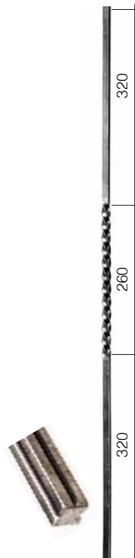
Art. ID118H2 \varnothing 12 x 12 mm H 900 mm
