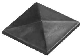
Art. ID1673 ∅ 30 x 30 mm Art. ID1674 ∅ 40 x 40 mm Art. ID1675 ∅ 50 x 50 mm Art. ID1677 ∅ 80 x 80 mm Art. ID1678 ∅ 100 x 100 mm
