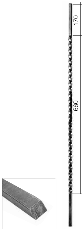
Art. ID11482 \varnothing 12 x 12 mm H 1000 mm
