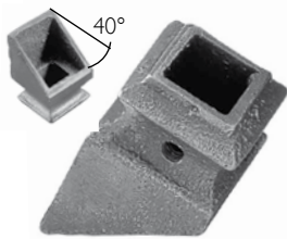
Art. ID14911 H 50 mm L 30 mm hole for \Phi 12 x 12 mm
