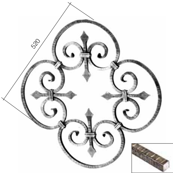
Art. ID243 12 x 12 mm 600 mm
